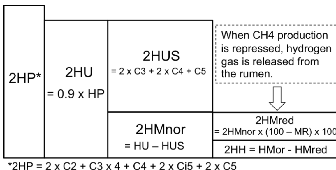
Figure 1. Calculation of 2H flowing into hydrogen gas.
