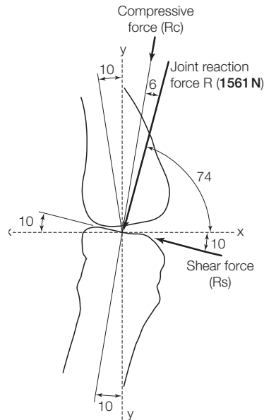
Fig. C8.12. Knee joint reaction, shear and compressive forces
