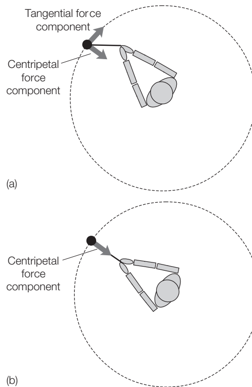
Fig. C7.2. The tension in the hammer wire and its components (a) during the increase in hammer head speed and (b) at maximum velocity before release
