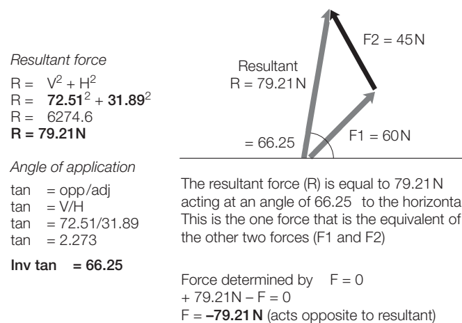
Fig. C5.6. Mathematical resolution of forces
