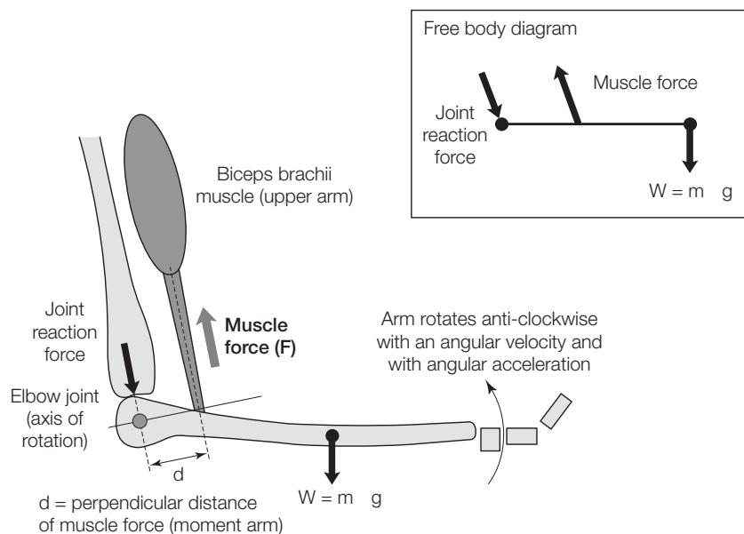
Fig. C2.5. Elbow flexion and extension movement
