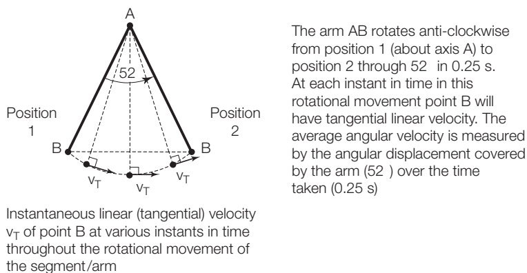
Fig. A4.8. Relationship between linear and angular components of motion
