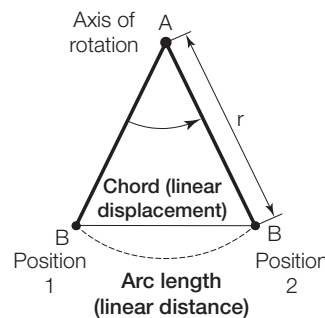
Fig. A4.4. Linear distance/displacement of a rotating object/point
