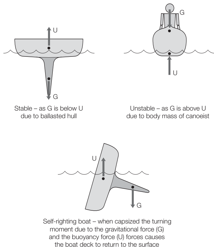
Fig. D6.2. Stability of yachts and canoes
