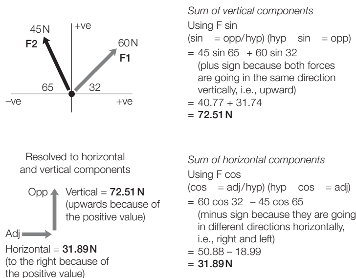
Fig. C5.5. Mathematical resolution of forces
