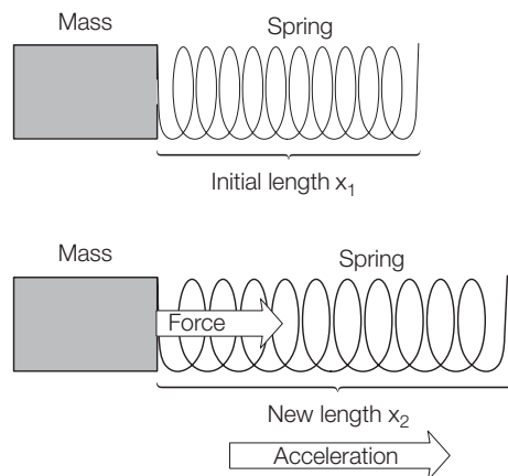
Fig. F4.1. A spring mass based accelerometer demonstrating the link between the deformation of the spring ( x_2 - x_1 ) and the acceleration ( a = k (x_2 - x_1)/\text{mass} ). Note that the acceleration of the accelerometer to the right requires the spring to lengthen until such time as the mass is experiencing a spring force sufficient to make it accelerate
